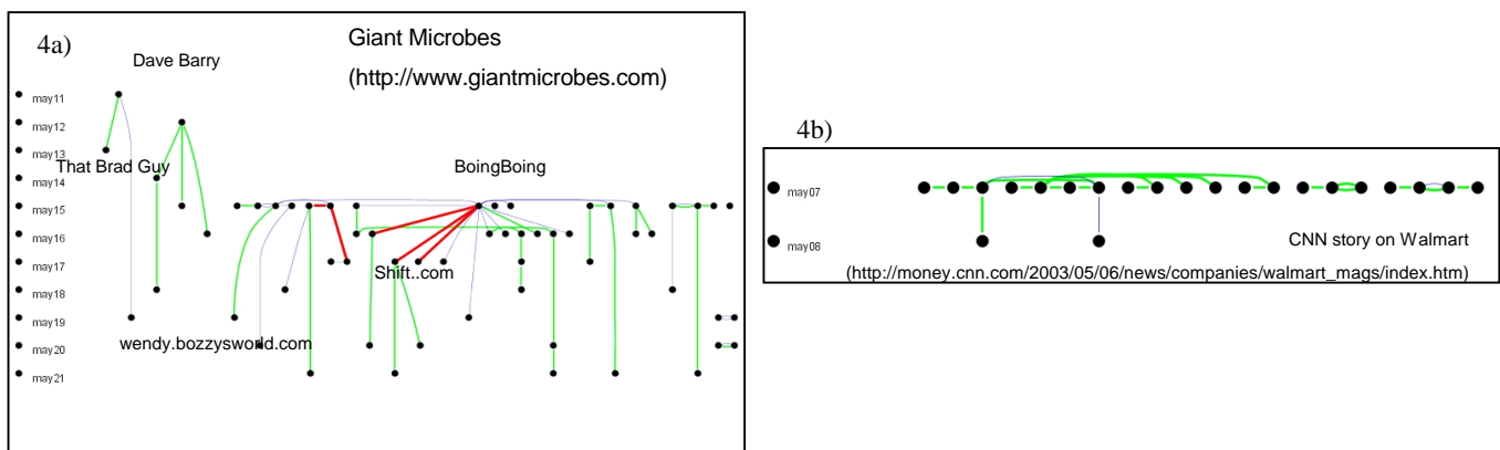
Figure 4a-b. Two depictions of the “most likely” infection trees determined by the algorithm described in Section 4. Thick red links (e.g. shift.com \rightarrow boingboing) are “via” links. Thin blue links (e.g. wendy.bozzysworld.com \rightarrow Dave Barry) are explicit links and the slightly thicker green links (e.g. thatbradguy.com \rightarrow Dave Barry) are inferred links. Figure 4a represents a longer running infection for the Giant Microbes site and 4b a short topical infection (a CNN news article).
